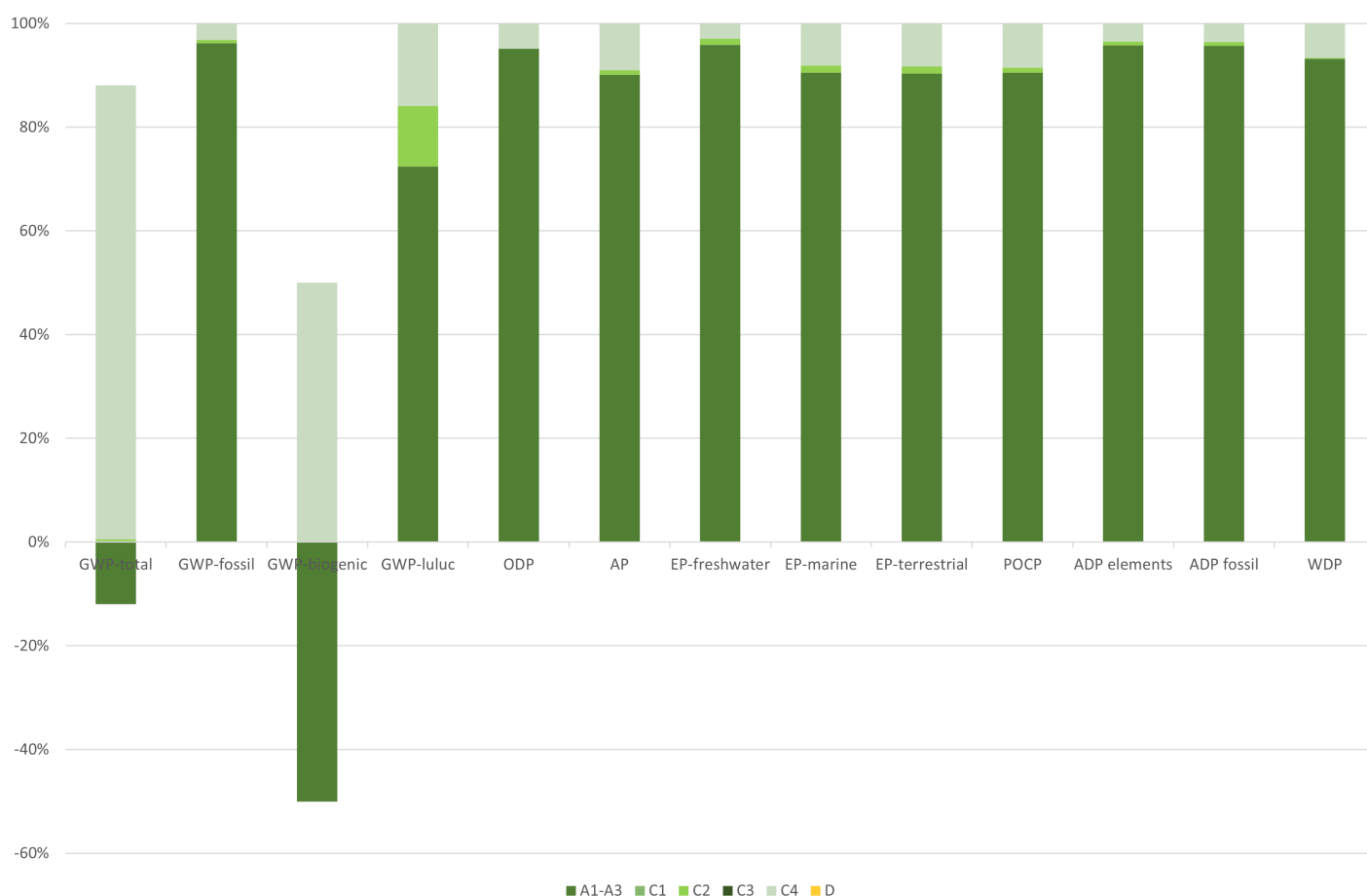
Hot-spot analysis of Heradesign ceiling panels Euroclass B
